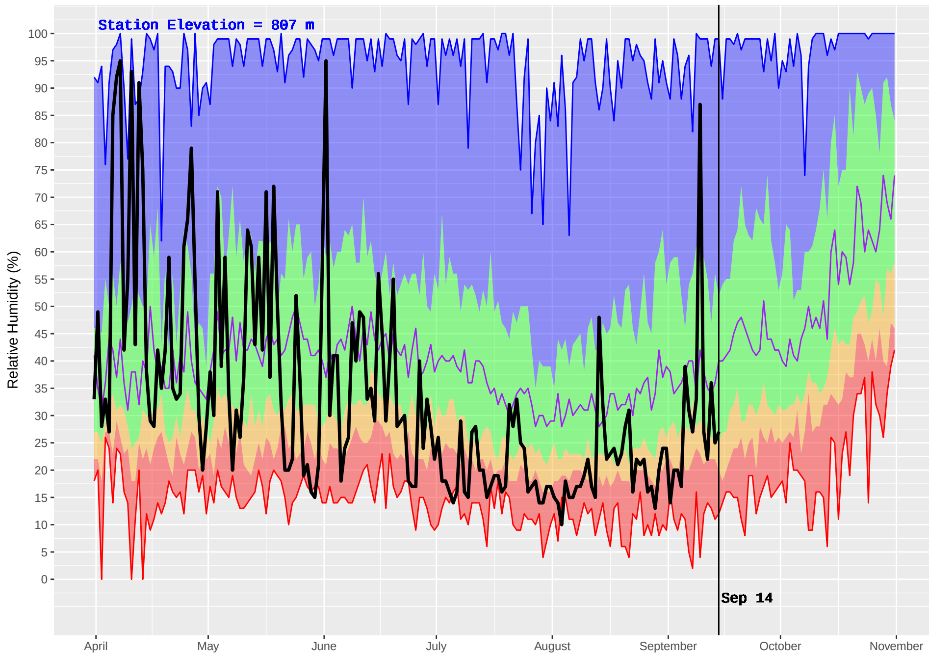
BEAVERDELL (390) : Historical (1970–2016) and Current (2017) Noon Relative Humidity
