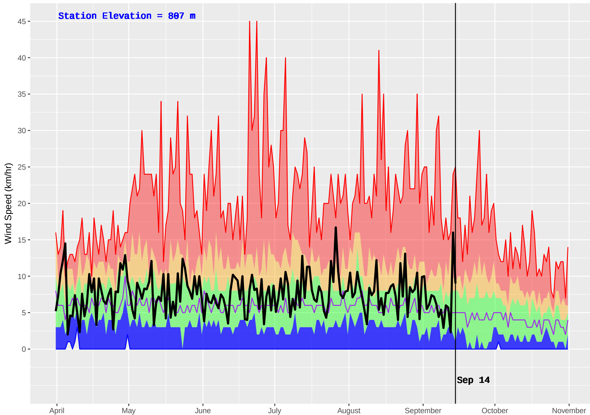
BEAVERDELL (390) : Historical (1970–2016) and Current (2017) Noon Wind Speed
