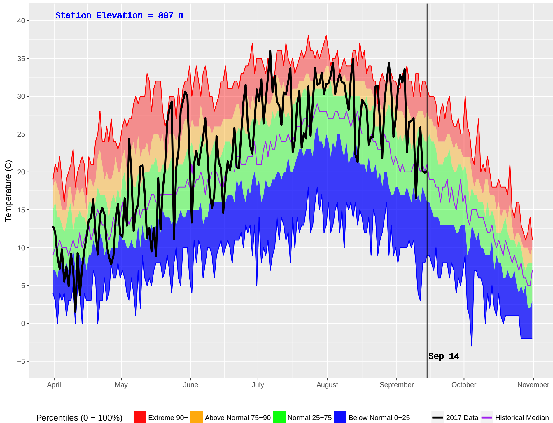
BEAVERDELL (390) : Historical (1970–2016) and Current (2017) Noon Temperature
