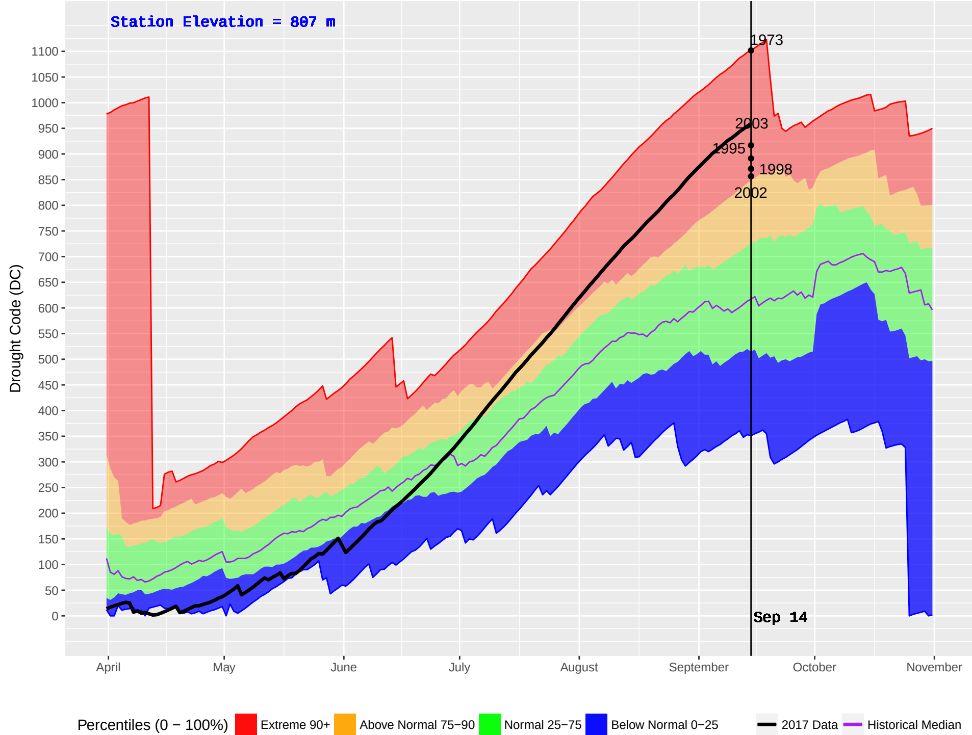
BEAVERDELL (390) : Historical (1970–2016) and Current (2017) Noon Drought Code (DC)
